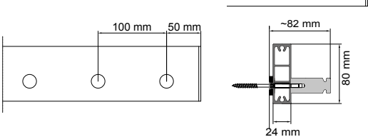
Haken 1330-06 hook 1330-06
